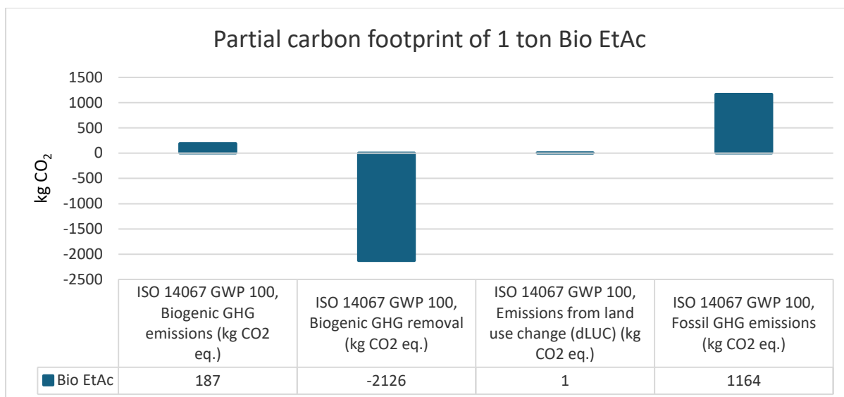
Figure 7. Partial carbon footprint for the production of 1 ton Bio EtAc.
